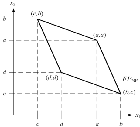
Figure 3(a). Set of feasible payoffs.
