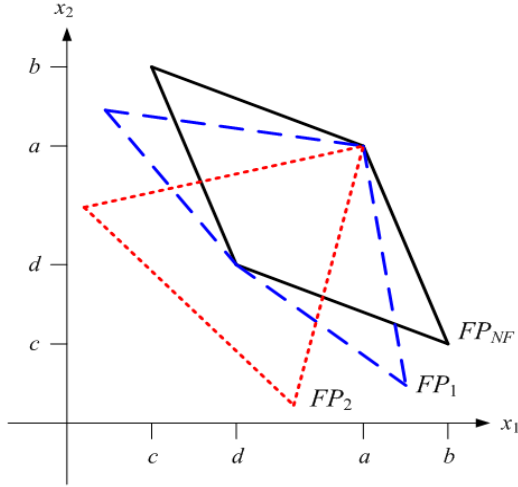
Figure 4. Set of feasible payoffs for \beta_i > 0 .
