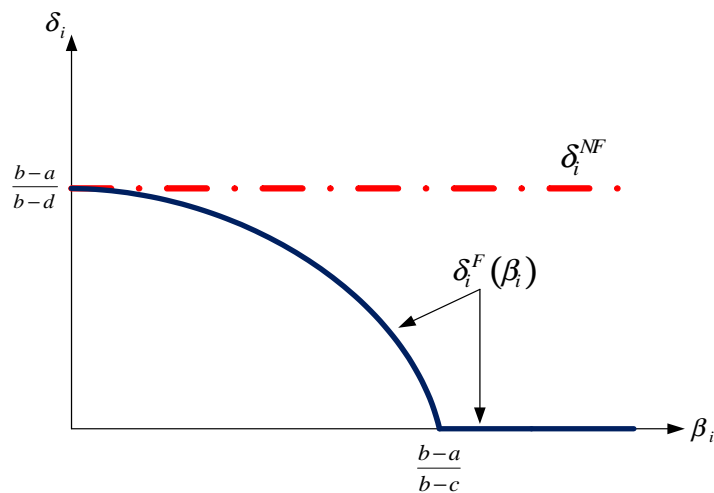
Figure 2. Discount factors \delta_i^F(\beta_i) and \delta_i^{NF} .
