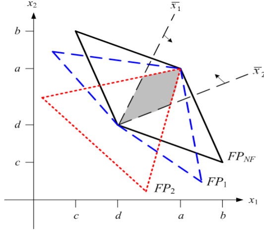
Figure 5. Effects of higher \alpha_i on the FIR set.
