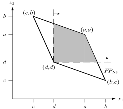
Figure 3(b). Individually rational payoffs.
